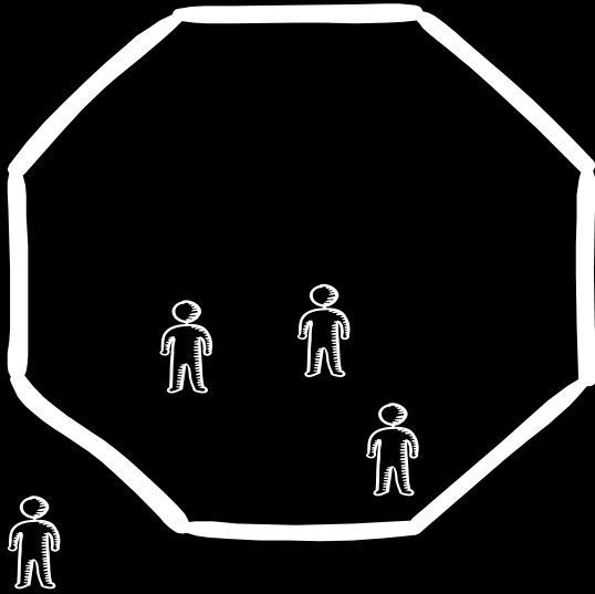
BOUNDED SET
