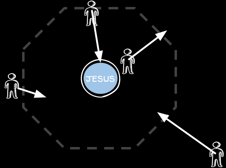
CENTERED SET
